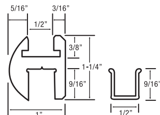
Deluxe Header Extrusion
