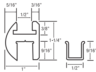
Deluxe Header Extrusion Snap-In Filler Insert
